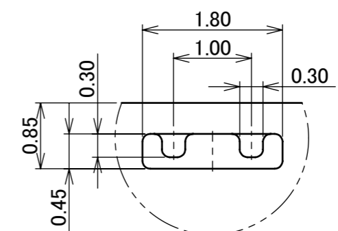
DETAIL L (S=15/1)
